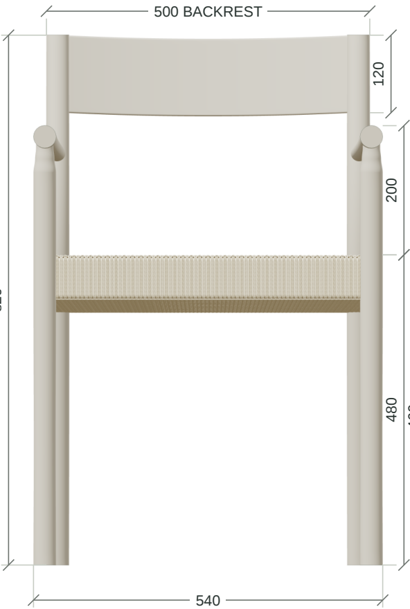
01 FRONT
